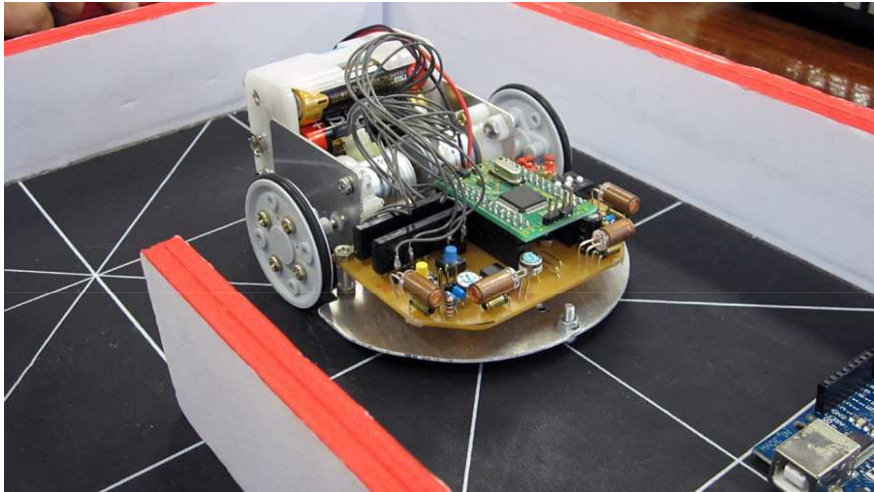
MICROMOUSE-LABYRINTTIROBOTTI
